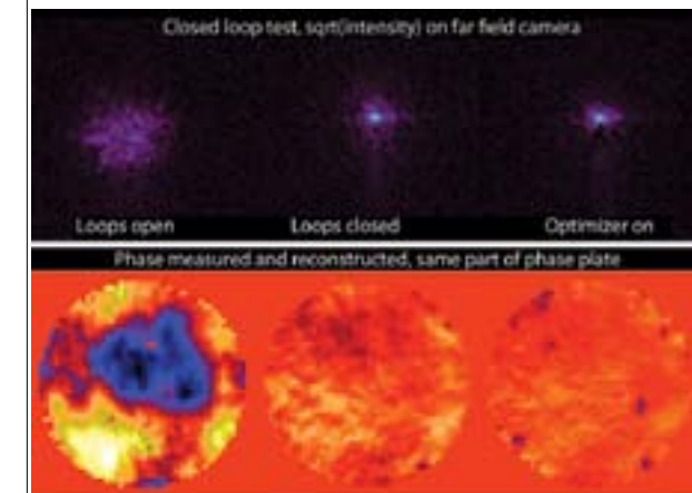
Figure 3. Focal plane images from the AO testbed at LLNL showing the image quality improvement with the AO loop closed and the real-time optimizer operating.
