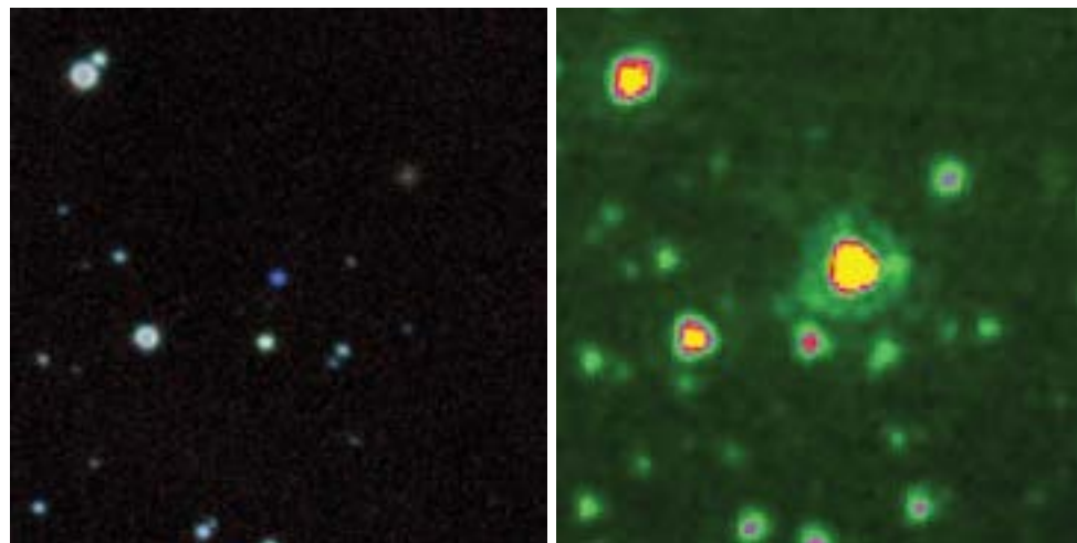
Figure 3. (left) Near-infrared, three-color image showing UGPS 0722-05 near the center. The blue color is characteristic of T dwarfs with strong absorption by methane. (right) An image at longer wavelengths taken with the Spitzer Space Telescope. Here the object appears as the brightest source in the field, and it is seen to have moved slightly to the right of center.
