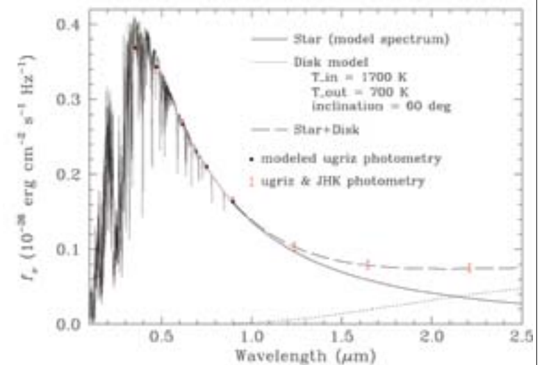
Figure 3. Photometric measurements using NIRI in the infrared, the Sloan Digital Sky Survey in the optical, and GALEX in the ultraviolet, compared to the best models of the star and the debris disk. The disk is most apparent at the longer wavelengths (above 1 micron) that NIRI measures.
