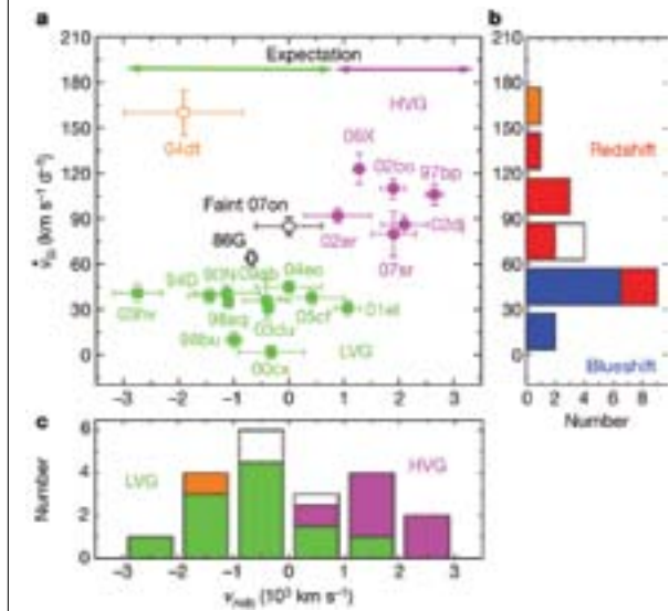
Figure 4. The viewing angle of the nebular emission ( v_{neb} ) is correlated with the velocity gradient of the ejecta ( v_{ej} ), which Maeda and colleagues explain as a consequence of asymmetric explosions of the Type Ia supernovae.
