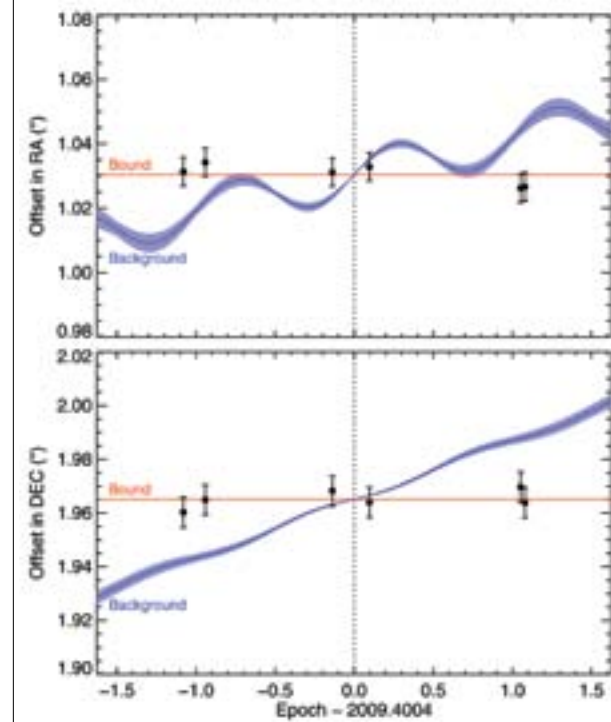
Figure 3. Position of the planet 1RXS 1609b relative to the primary star as a function of time (black points). The relative position shows no change over time, indicating that the planet is bound to the star. Had the planet been a distant, unrelated background star, the relative position would have followed the blue curve. The RA and DEC plotted on the figure are coordinates on the celestial sphere similar to longitude and latitude, respectively, on the surface of the Earth.
