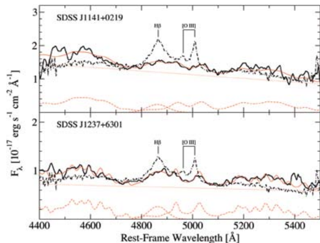
Figure 5. Observed near-infrared spectra of two high-redshift, weak emission line quasars (solid black lines) correspond to the restframe optical emission. These sources show very different spectra than typical quasars (dot-dashed lines), especially around the emission lines (noted as H \beta and [O III]).
