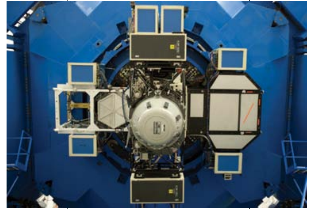
Figure 3. GNIRS on the uplooking port at Gemini North, seen from below.
