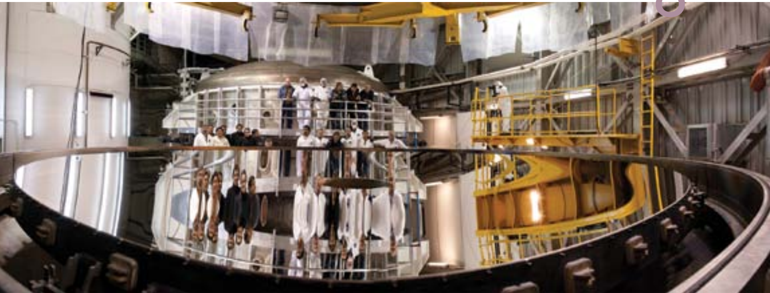
Figure 1. The mirror coating and support team reflected in the fresh coating on the Gemini South mirror shortly after it emerged from the coating chamber seen in the background.
