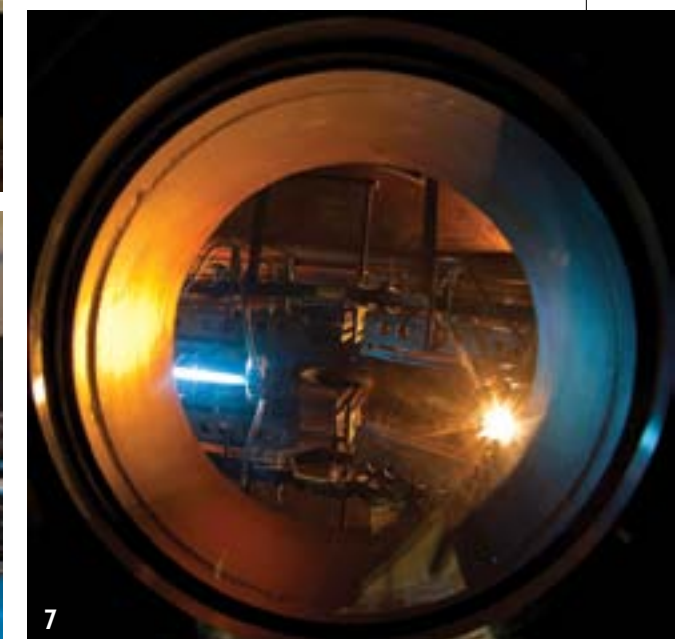
Figures 2 - 7. Counterclockwise from top right: 2) primary mirror shortly after removal of mirror cell, 3) application of paper towels to absorb acid used to strip off the old coating, 4) cleaning of mirror after removal of the old coating, 5) final cleaning of mirror with carbon dioxide snow prior to coating, 6) concurrent work on Cassegrain rotator, 7) view of mirror during coating with magnetron (left) applying a coating layer.
