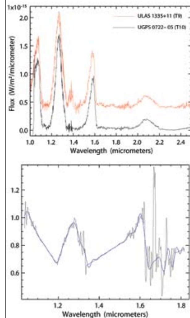
Figure 2. (top) Gemini spectrum of the T10 dwarf UGPS 0722-05 (black line). One of the three known T9 dwarfs is shown in red for comparison. (bottom) A ratio spectrum of the T10 dwarf divided by the average of the three T9 dwarfs. It shows more clearly that the water and methane broad-absorption troughs to either side of the peaks at 1.27 and 1.59 microns are deeper in this object. The spectra are reproduced from Monthly Notices of the Royal Astronomical Society Letters.
