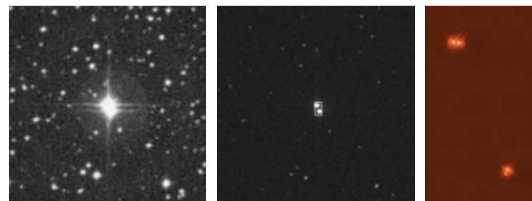
Figure 5. (left) Digital Sky Survey 2 (DSS 2) image of HIP 43947, showing the binary nature of this quite bright star. (center) 2MASS infrared (K band) image at the same scale as the DSS 2 image with a box indicating the approximate area covered by the Gemini NICI observations. (right) NICI infrared (K band) image, revealing the binaries that make up the quadruple star system.
