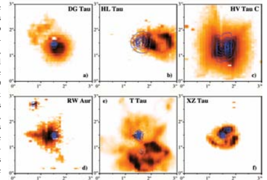
Figure 3. Adaptive optics observations with NIFS revealed the detailed structure of molecular hydrogen gas surrounding six protostars. The gas velocities measured by NIFS traced multiple components within the gas cloud, showing signs of jets, winds, and disks of accreting matter. Figure courtesy of Tracy Beck
