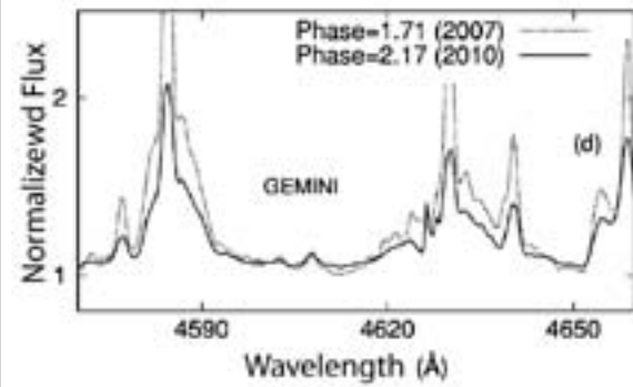
Figure 2. The most recent GMOS-S spectra of Eta Carinae (from 2010) show stellar-wind emission lines that are about two times weaker than those that had been observed in 2007. These spectral extractions show the effect on blends of permitted and forbidden ionized iron and chromium.
