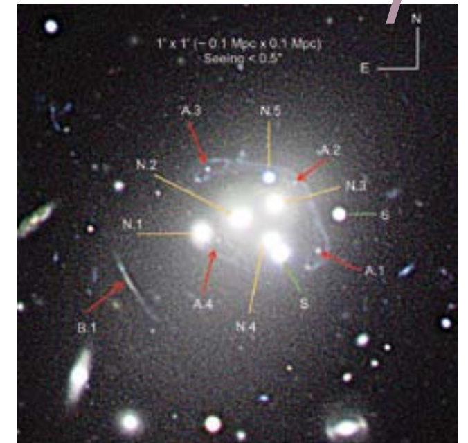
Figure 1. Color-composite image (g', r', and i') of the multi-component BCG in Abell 3827. The five galaxies that form the BCG are labeled N.1 to N.5. The strong gravitational lensing features are also seen in the image.
