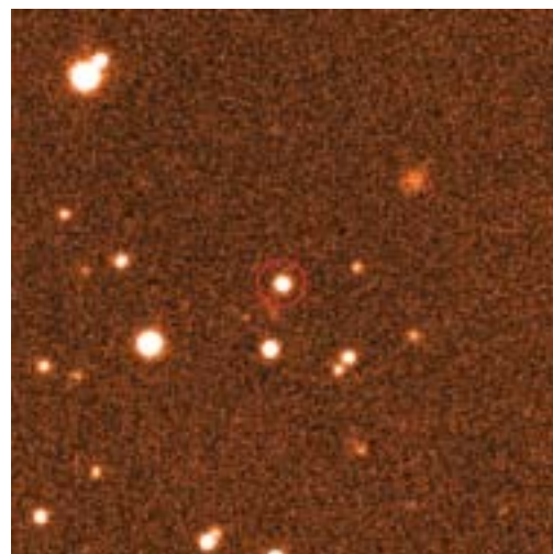
Figure 1. (top) UKIDSS discovery image of the star field around UGPS 0722-05 (circled), taken in November, 2006. (bottom) The image of the same field taken with the 2MASS survey in 1998. The brown dwarf had moved 8 arcseconds in the intervening years.
