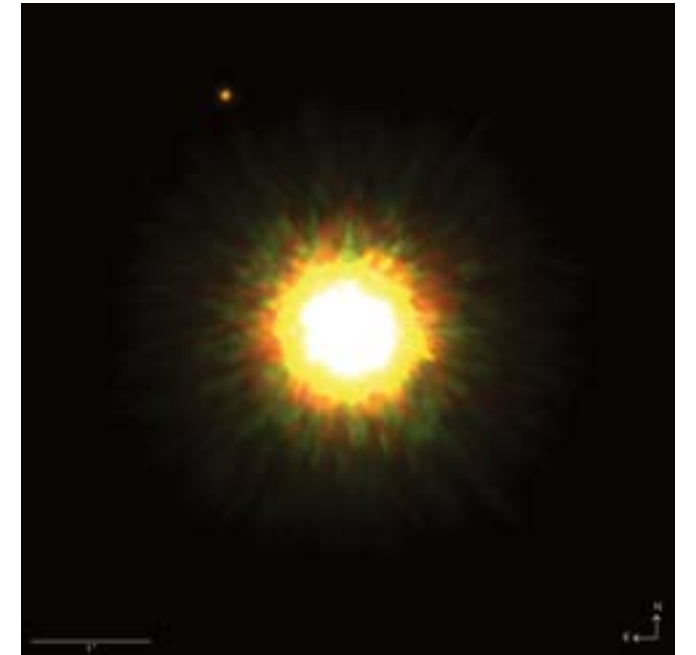
Figure 1. Image of 1RXS J160929.1-210524 and its ~ 8 Jupiter-mass companion. This image is a composite of J-, H-, and K-band, near-infrared images obtained with the Gemini North adaptive optics system and the NIRI camera.
