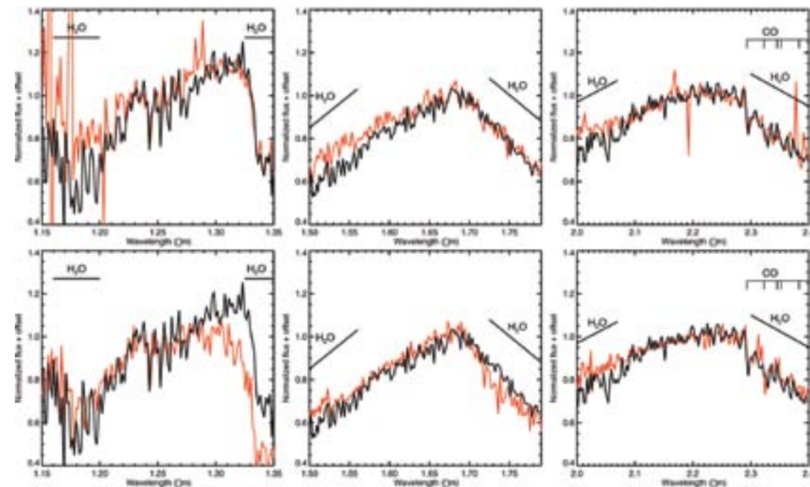
Figure 2. The spectrum of the planet obtained with the NIRI and NIFS instruments at Gemini is shown in black. On the top row, the spectrum is compared with that of a young, slightly warmer, more massive, free-floating, brown dwarf that is also a member of the Upper Scorpius association (red, from Lodieu et al., 2008). On the bottom row, the spectrum is compared with a model spectrum of temperature 1800 K and low surface gravity (red, from DRIFT PHOENIX models, Witte et al., 2009, Helling et al., 2008).
